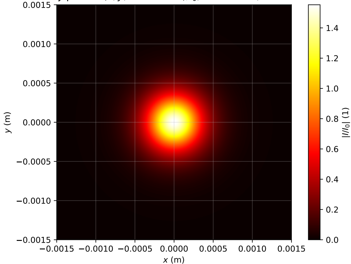
Intensity profile I(x, y, z = 3.105m)/I_0 , Pin=0.9Pcr, artificial time
